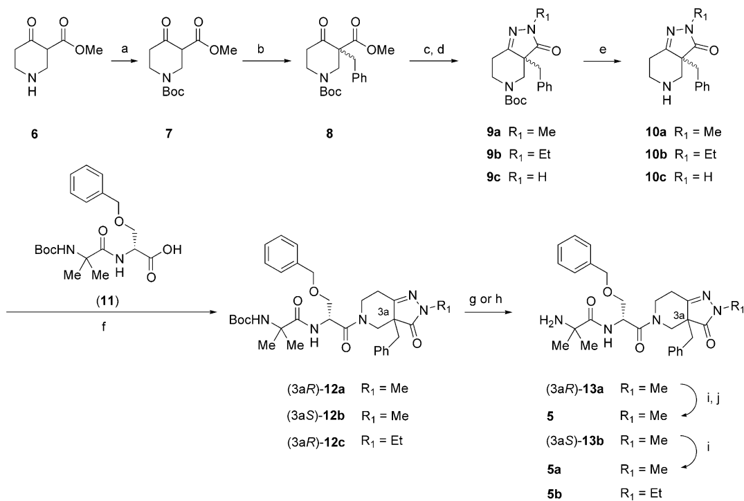
Scheme 1. Syntheses of GHSs 5 , 5a and 5b . Reagents and conditions: (a) \text{Boc}_2\text{O} , DMAP, \text{CH}_2\text{Cl}_2 , 0^\circ\text{C} ; (b) NaH, \text{PhCH}_2\text{Br} , DMF; (c) \text{R}_1\text{NHNH}_2 , EtOH, reflux; (d) toluene, reflux; (e) TFA, \text{CH}_2\text{Cl}_2 , 0^\circ\text{C} or concd HCl, EtOH; (f) HOAt, EDC, \text{NEt}_3 , \text{CH}_2\text{Cl}_2 , 0^\circ\text{C} ; (g) TFA, \text{CH}_2\text{Cl}_2 , 0^\circ\text{C} ; (h) concd HCl, EtOH; (i) (L)-tartaric acid, MeOH; (j) EtOAc, reflux.
