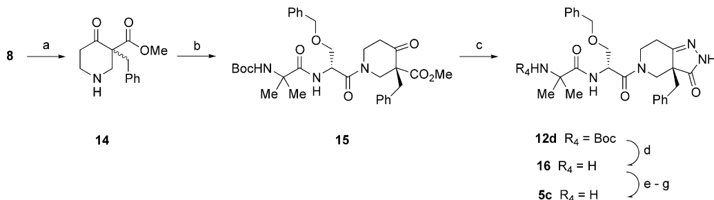
Scheme 2. Synthesis of GHS 5c . Reagents and conditions: (a) TFA, CH 2 Cl 2 , 0 °C; (b) 11 , EDC, HOAt, CH 2 Cl 2 , 0 °C; (c) NH 2 NH 2 ·H 2 SO 4 , NaOAc, EtOH, 78 °C; (d) concd. HCl, EtOH; (e) saturated aqueous NaHCO 3 ; (f) (L)-tartaric acid, MeOH; (g) EtOAc, 80 °C.
